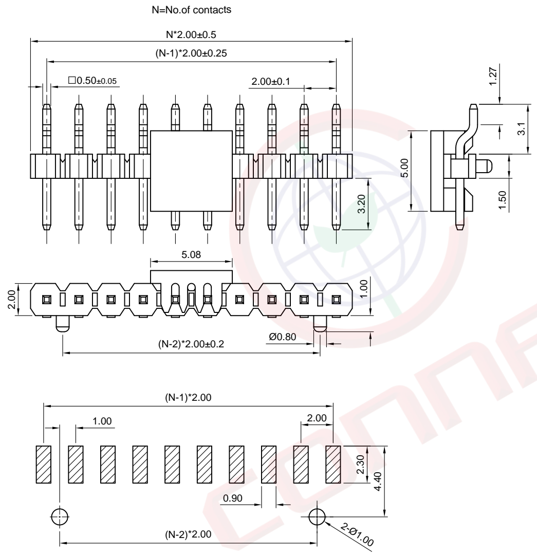
Recommend PCB Layout (Tolerance=±0.05)
