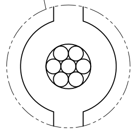
Stranded Type DETAIL (SCALE 8:1)
