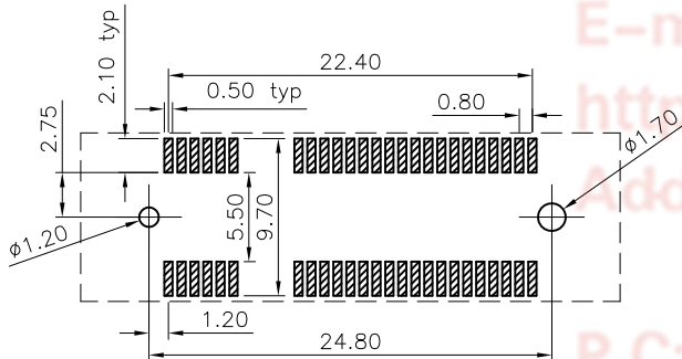
RECOMMEND PCB LAYOUT
